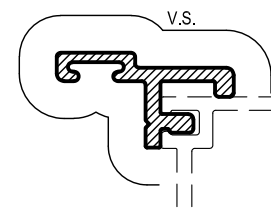
MFA29 MEETING STILE ADAPTOR Mass. 0,215 Kg/m Anod. Per. 100 Paint Per. 100
