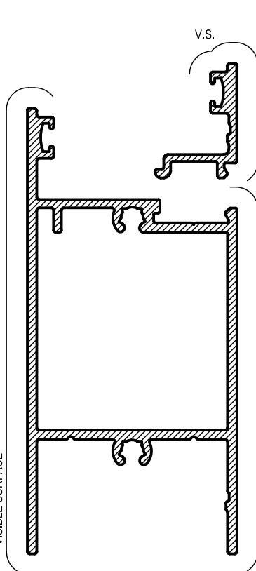
AFD20 40mm DG RAIL BEAD Mass. 0,190 Kg/m Anod. Per. 100 Paint Per. 100
