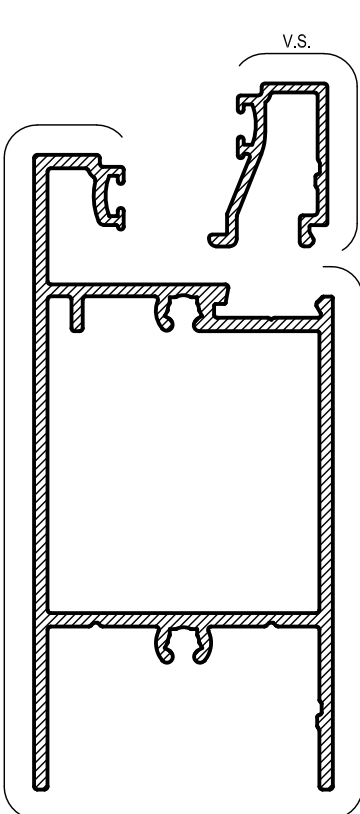
AFD27 40mm SQUARE RAIL BEAD Mass. 0,218 Kg/m Anod. Per. 125 Paint Per. 100
