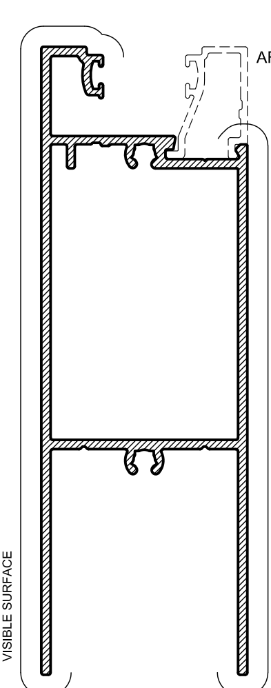
** AFD23 40mm SG DEEP RAIL Mass. 1,650 Kg/m Anod. Per. 481 Paint Per. 243
