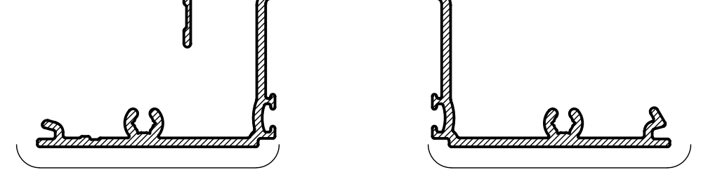
AF313 DG FRAME ADAPTOR Mass. 1,003 Kg/m Anod. Per. 440 Paint Per. 100 Ixx = 406.81 x 10 3 mm 4 Iyy = 44.01 x 10 3 mm 4
