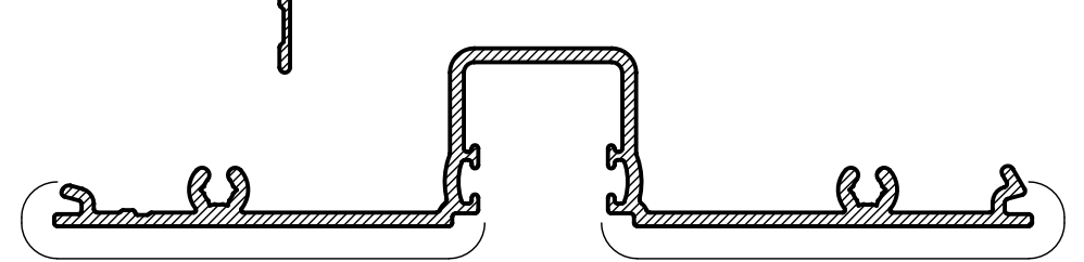
AF213 GLAZING ADAPTOR Mass. 0,930 Kg/m Anod. Per. 408 Paint Per. 102 Ixx = 383.34 x 10 3 mm 4 Iyy = 16.52 x 10 3 mm 4
