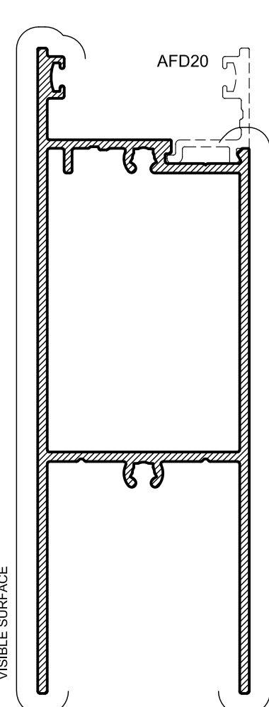
** AFD26 40mm DG DEEP RAIL Mass. 1,595 Kg/m Anod. Per. 452 Paint Per. 237
