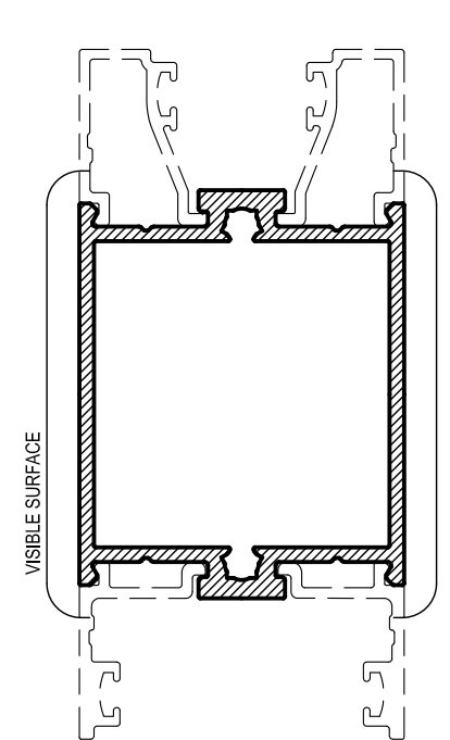
AFD15 40 x 85 MID RAIL Mass. 0,963 Kg/m Anod. Per. 212 Paint Per. 100
