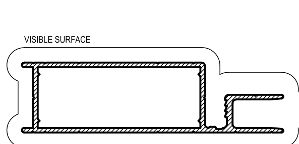
SD2 DOOR FRAME Mass. 0,591 Kg/m Anod. Per. 228 Paint Per. 194
